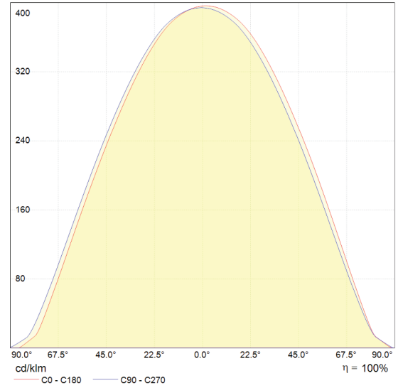
CONICAL DIAGRAM
