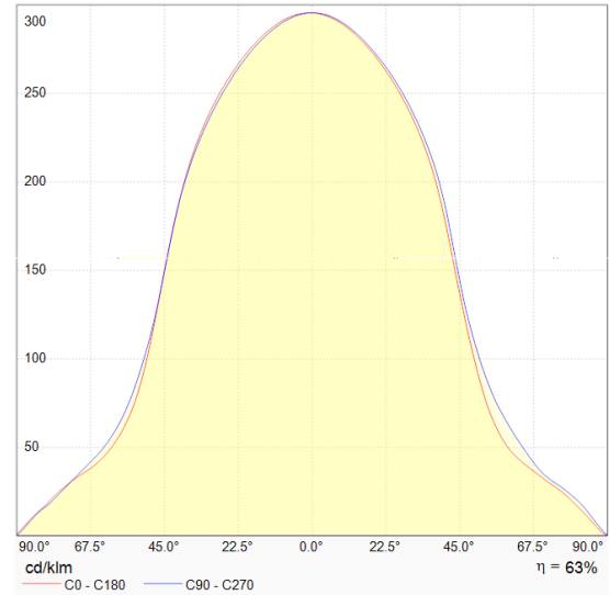
CONICAL DIAGRAM
